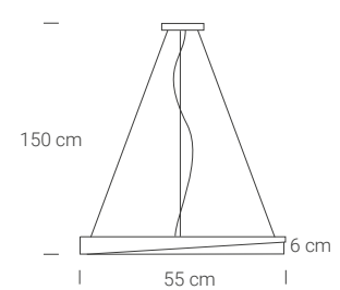
Loola sospensione Loola suspension
